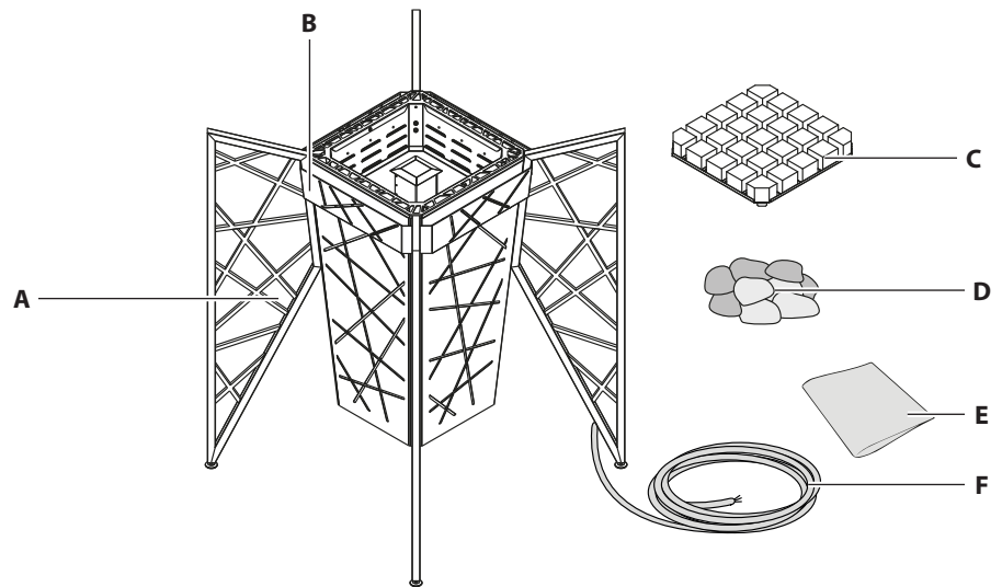
General view of the sauna heater and the scope of delivery
