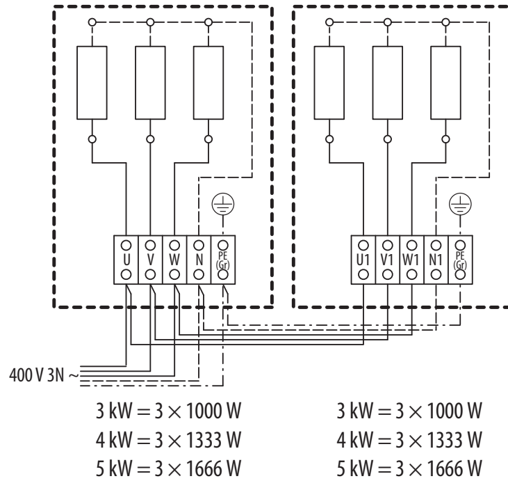
Connection diagram, heater output 6 kW, 8 kW, 10 kW
