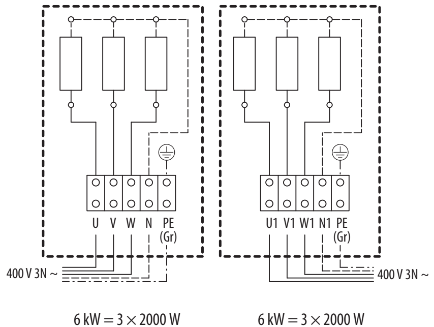
Connection diagram, heater output 12 kW
