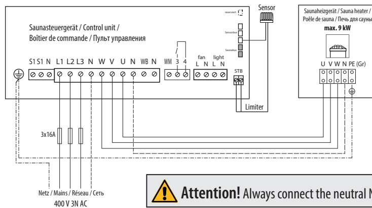
Connection example for EOS EmoTec / EmoStyle / EmoTouch control units
